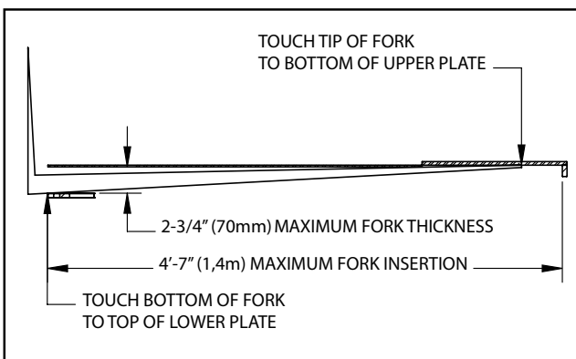
Fig. 5c - Fork Requirements for Compatibility with SkyORB Base Forklift Pockets
